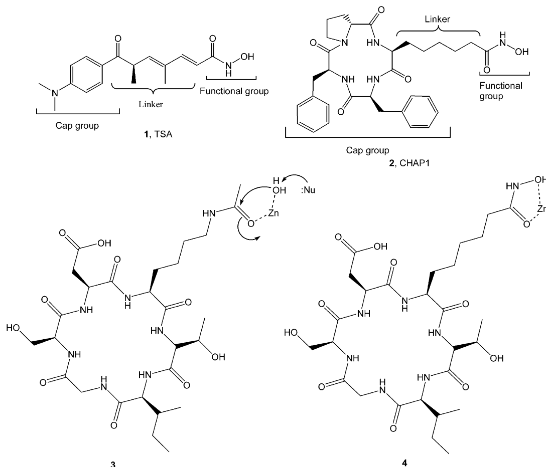
Figure 1. Reported and proposed HDAC inhibitors and substrate.
