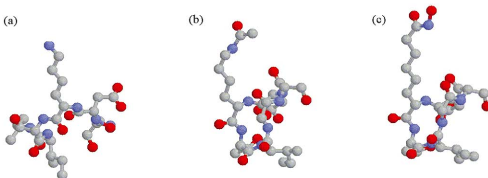
Figure 2. (a) X-ray structure of \alpha -tubulin fragment (-Ser- Asp -Lys 40 - Thr- Ile-Gly-); (b) Calculated conformation of compound 3 . (c) Calculated conformation of compound 4 .
